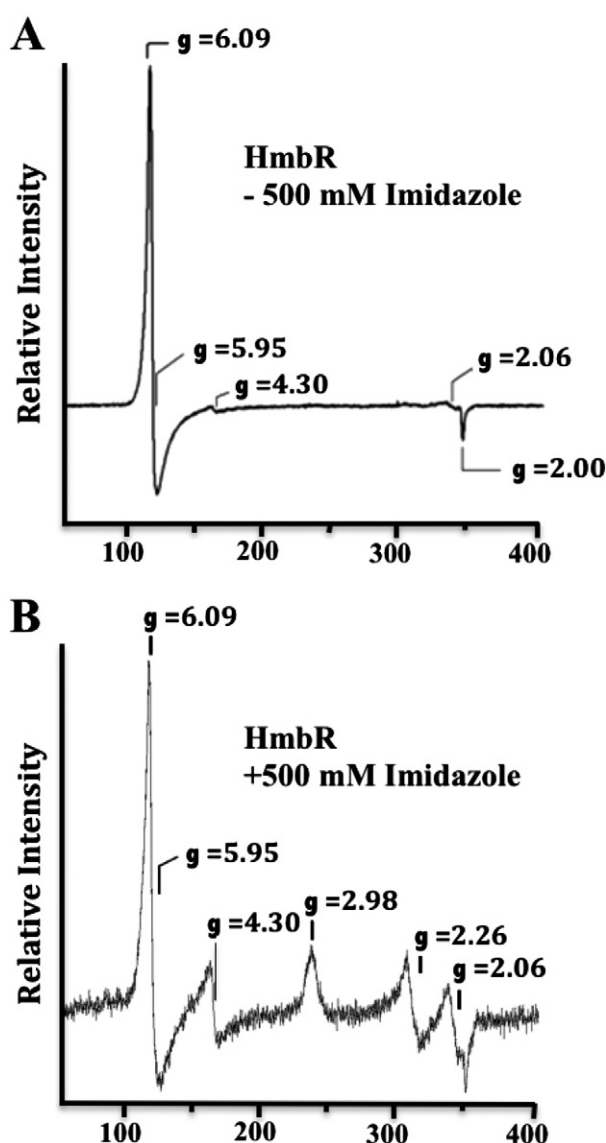
Fig. 3. Electron paramagnetic resonance spectra of HmbR. EPR spectra were recorded on samples containing approximately 200 \mu\text{M} of HmbR in sample buffer (20 mM phosphate, pH 7.4, and Anzergent TM 3–14) either without imidazole (Panel A), or in the presence of 500 mM imidazole (Panel B). All data were collected using a Bruker ESP300D spectrometer equipped with an Oxford Instruments ESR-900 helium flow cryostat to maintain the temperature of the samples at 10 K. The modulation amplitude was 6.477 G with a modulation frequency of 100 kHz. The microwave frequency and power were 9.6 GHz and 5 mW, respectively. The signal at g = 4.3 is attributed to minute contamination of the protein sample by rhombic iron(III). The feature at g = 2.06 is attributed to copper contamination of the EPR cavity.
