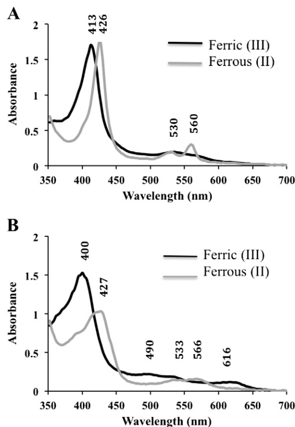
Fig. 1. Electronic Absorption Spectra of HmbR. Purified HmbR in sample buffer (20 mM phosphate, pH 7.4, 500 mM NaCl) was subjected to UV-visible absorption scans either A ) as purified (with 500 mM imidazole) or B ) after removal of imidazole. Black lines represent the spectra of samples in the ferric state, and gray lines represent the spectra of samples reduced to the ferrous state by the addition of 5 mM sodium hydrosulfite to the sample. Each spectrum was obtained using 1.5 \mu\text{L} of protein at approximately 35 mg/mL on a nanodrop (ND-1000) spectrophotometer. Soret, \alpha , and \beta peaks are indicated by their respective wavelengths within the graphs.
