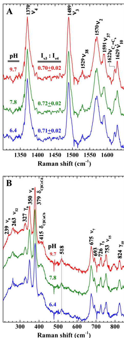
Fig. 4. Resonance Raman spectrum of HmbR. Resonance Raman of HmbR showing the A) high frequency and B) low frequency spectra. Each panel has three spectra (bottom, middle, and top) corresponding to different buffers (MES, Tris, or CAPS) and pH conditions (6.4, 7.8, and 9.7), respectively. Samples were prepared in 0.05% Anzergent™, 300 mM NaCl, and 100 mM of the indicated buffer. Data were obtained using a 406.7 nm emission from a Kr + laser using a power of 14 mW, a 135° backscattering geometry, and spun at 20 Hz in 5 mM NMR tubes at room temperature to avoid laser induced degradation. The laser beam was calibrated against Raman frequencies of toluene and DMF, and focused to a line on the spinning NMR tubes. The identity of certain peaks is indicated in each graph.
